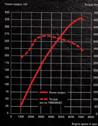
5.2 V10-FSI Engine
